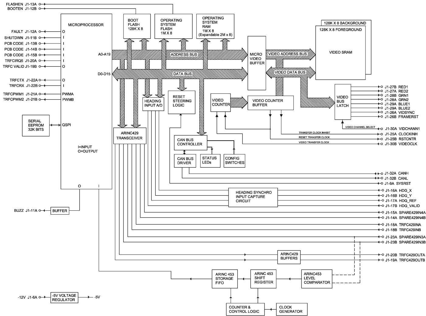
Figure 16 KAC 504 TRFC Processor Board Block Diagram
