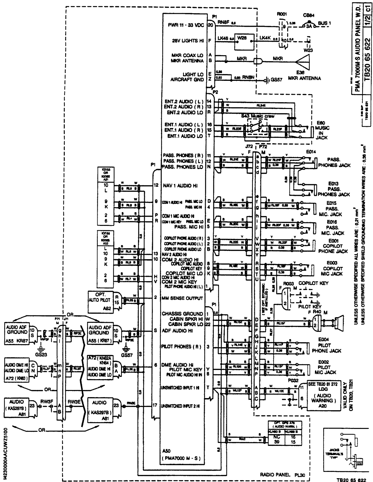
Figure II.6.23.10.10K - BOITE DE COMMANDE AUDIO PMA 7000 M.S. PMA 7000 M.S.AUDIO CONTROL BOX OPT10 23001A
